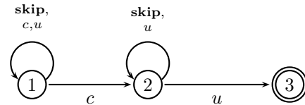
Figure 5: The automaton for the obs tracematch.
