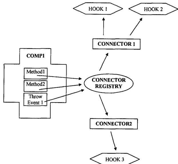
Figure 10: JAsCo architecture.
