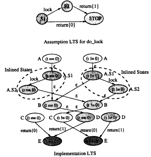
Figure 5. LTS for do_lock and M_{Imp} .
