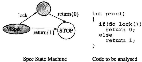
Figure 1. The example M_{Spec} and proc .
