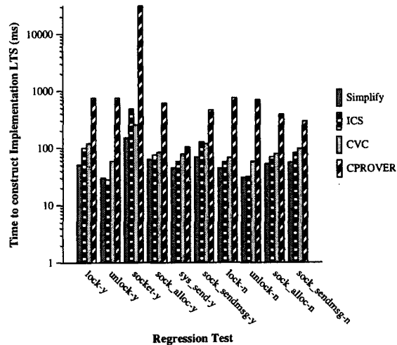
Figure 7. Time to construct M_{Imp} .
